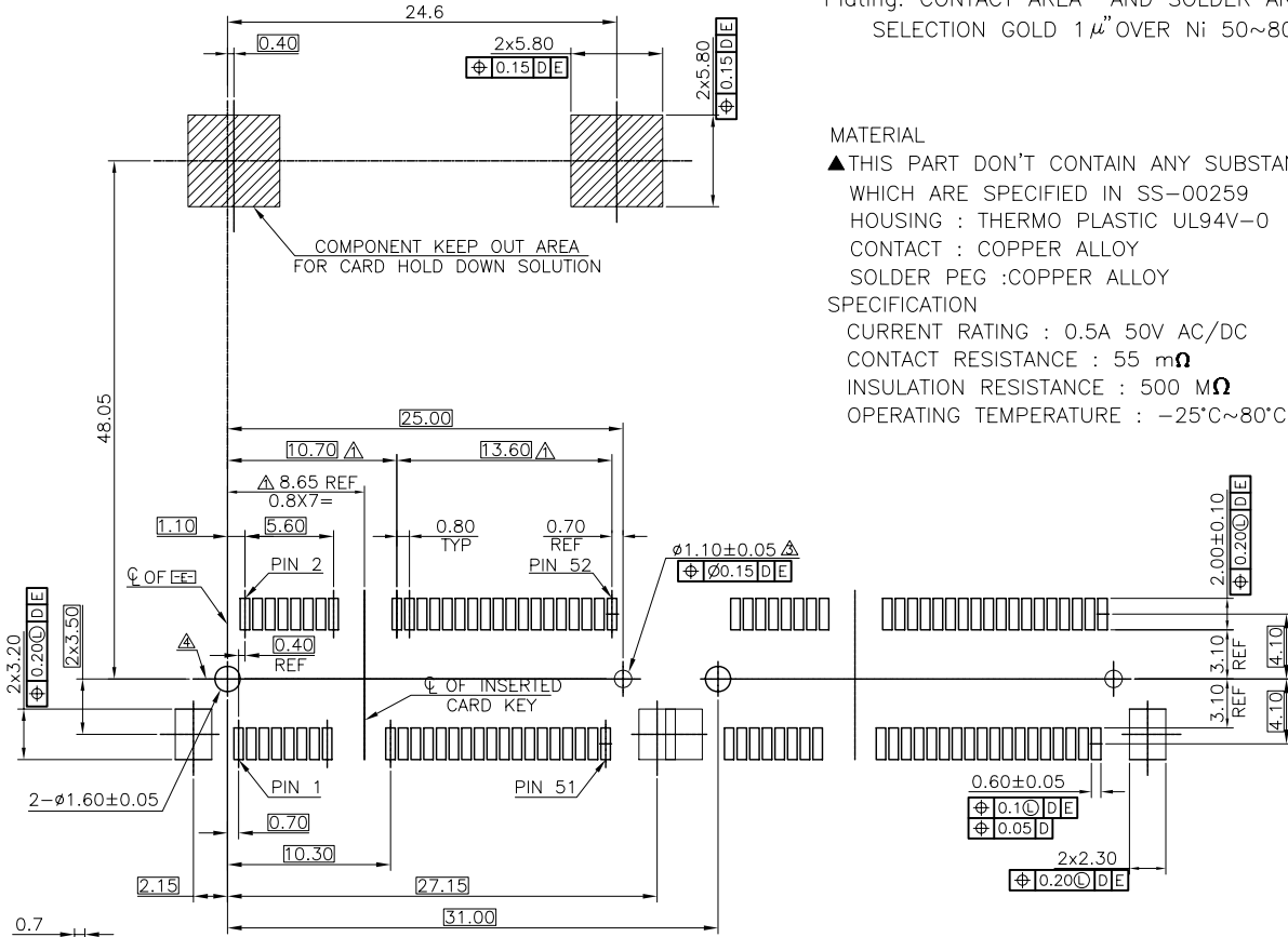
RECOMMENDED P.C.BOARD PATTERN LAYOUT (SIDE BY SIDE)
