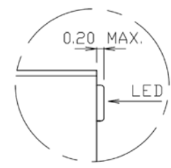
DETAIL W
