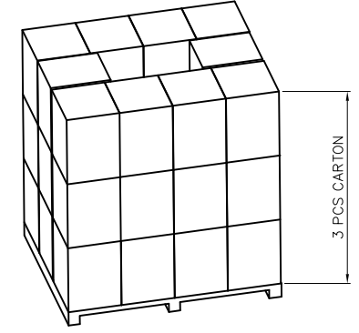
STACK DIAGRAM
