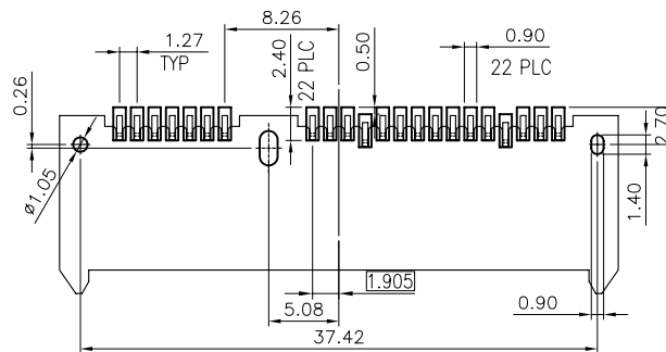
VIEW D
