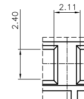
VIEW C SCALE 2:1
