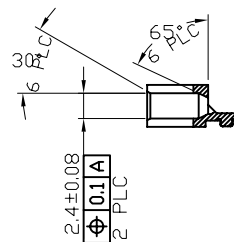
SECTION Y-Y
