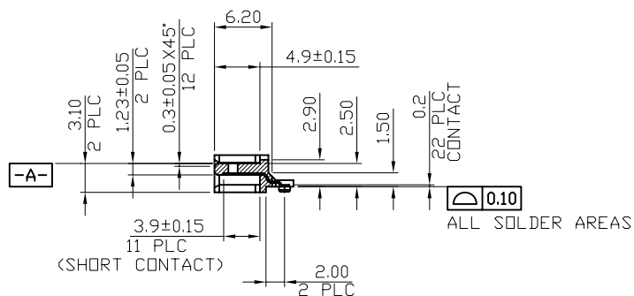
SECTION Z-Z
